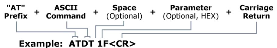
Figure B-25 Syntax for sending AT Commands:
