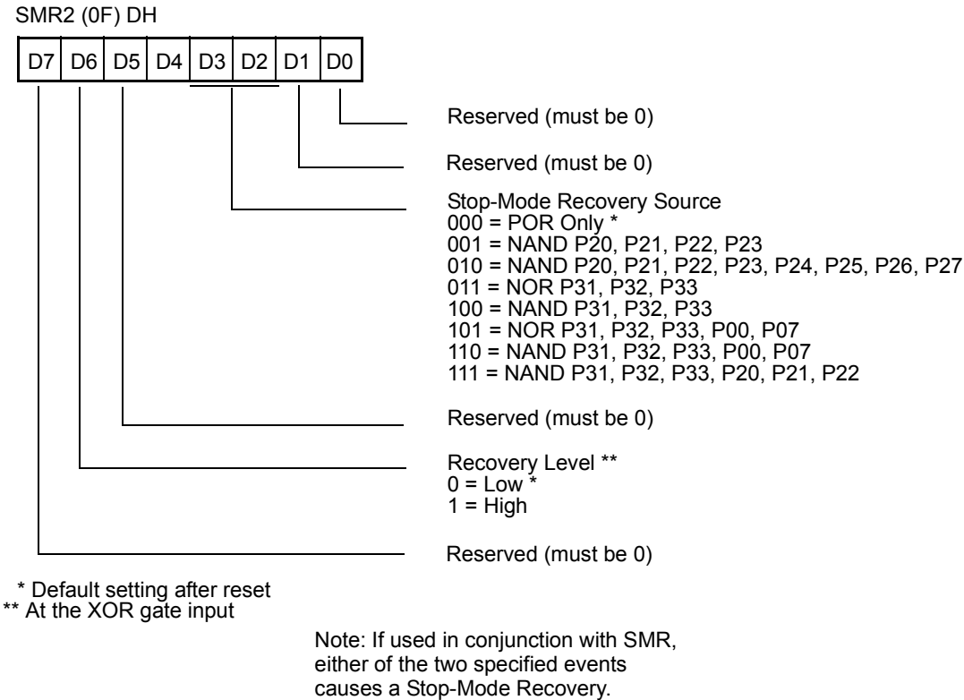
Figure 17. Stop-Mode Recovery Register 2—(0F) 0DH: D2–D4, D6 Write Only
