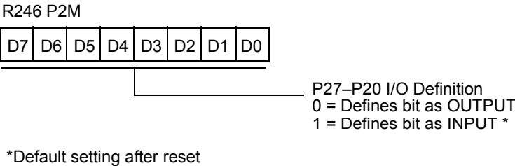
Figure 20. Port 2 Mode Register—F6H: Write Only
