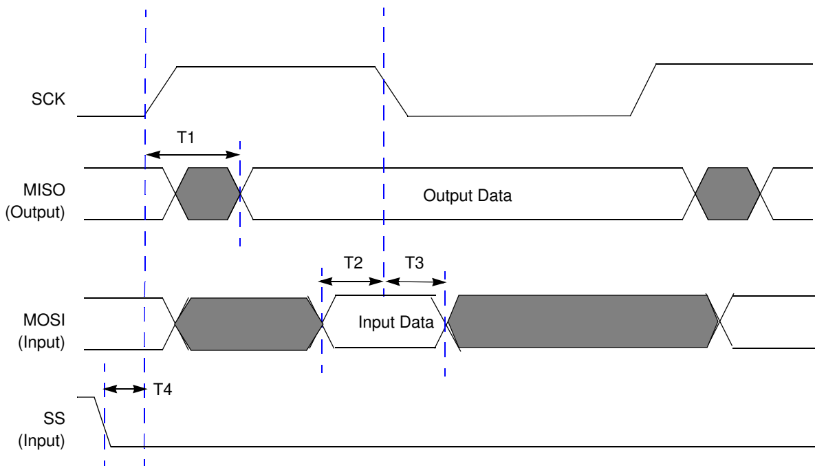
Figure 52. SPI SLAVE Mode Timing
