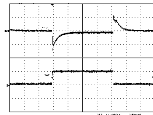
Figure 2.5 100mA to 2A Load Step ( V_{CC} = 12\text{V} , V_{OUT} = 3.3\text{V} )
