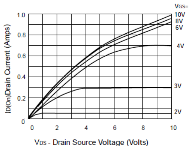
Saturation Characteristics
