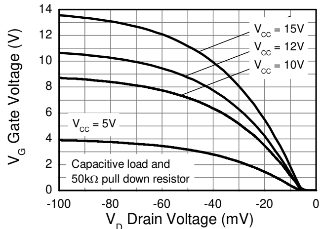
Transfer Characteristic
