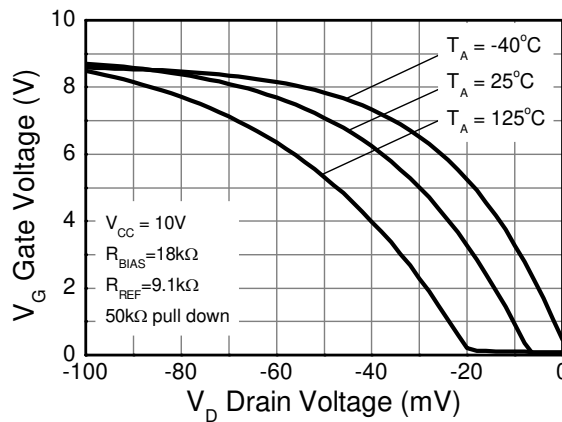
Transfer Characteristic
