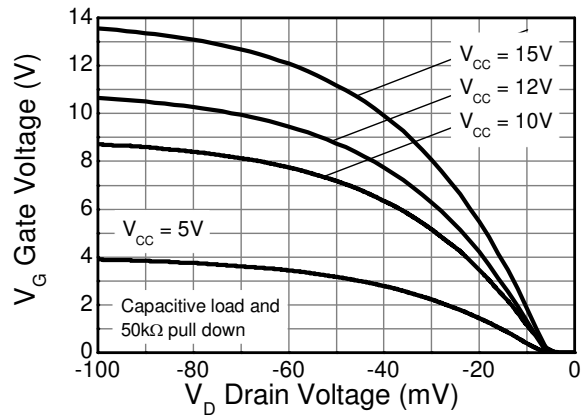
Transfer Characteristic
