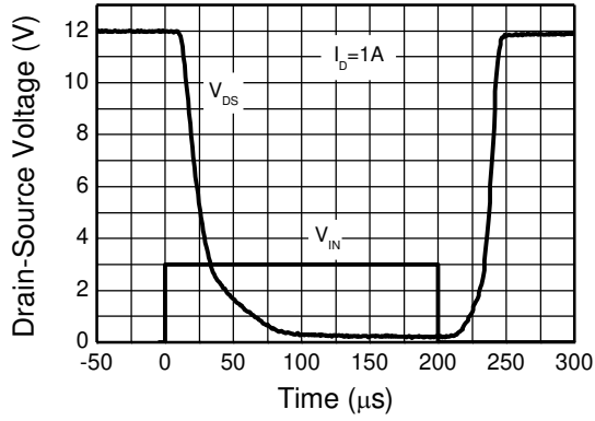
Switching Speed
