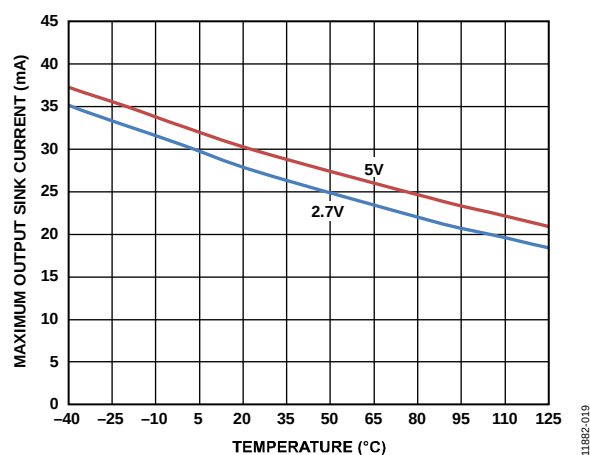
Figure 20. Maximum Output Sink Current vs. Temperature
