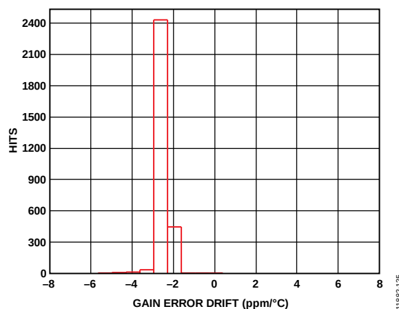
Figure 26. Gain Error Drift Distribution
