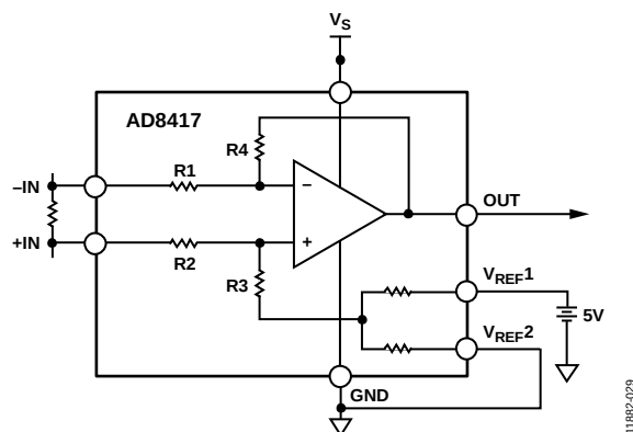
Figure 31. Split External Reference
