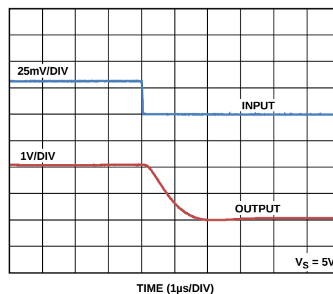
Figure 14. Fall Time ( V_S = 5\text{ V} )
