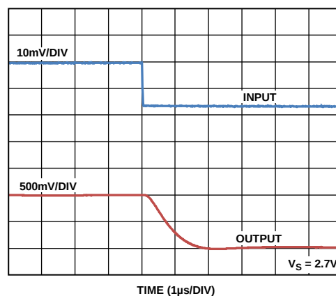
Figure 13. Fall Time ( V_S = 2.7\text{ V} )
