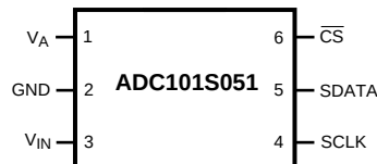
Figure 1. WSON and SOT-23 Packages See Package Numbers NGF0006A and DBV0006A
