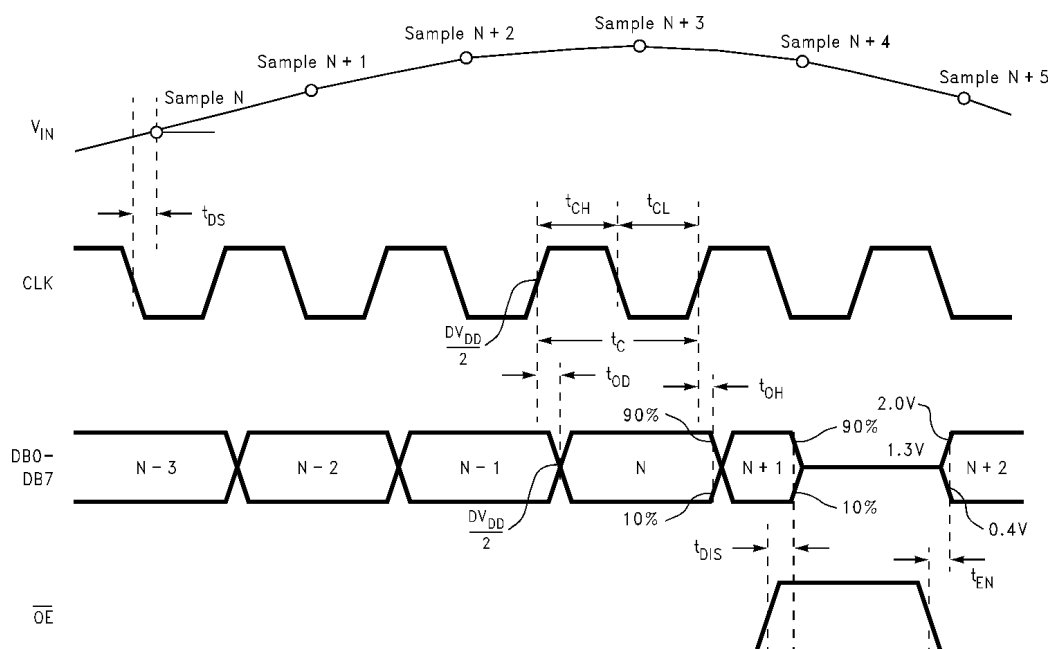
Figure 24. Timing Diagram
