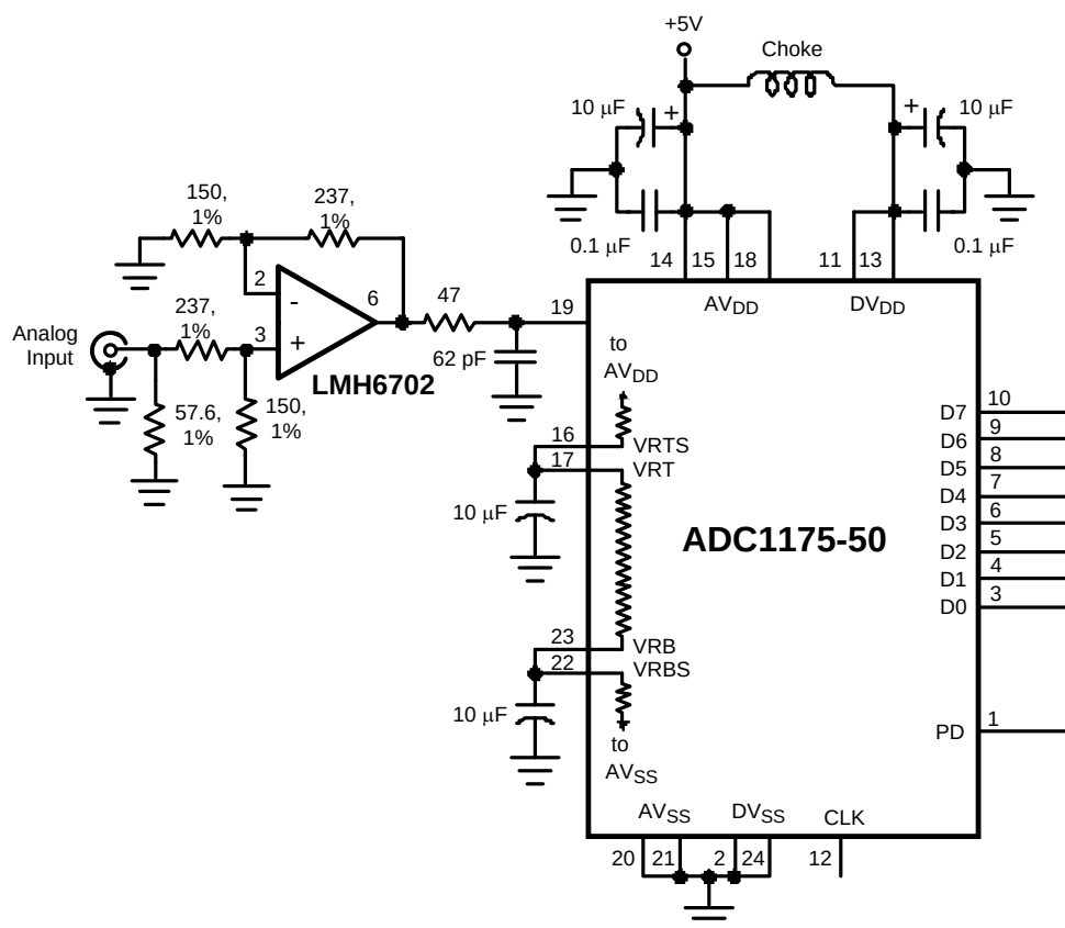
Figure 17. Driving the ADC1175-50
