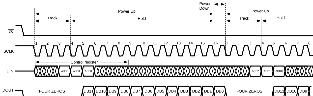
Figure 1. ADC128S052 Operational Timing Diagram
