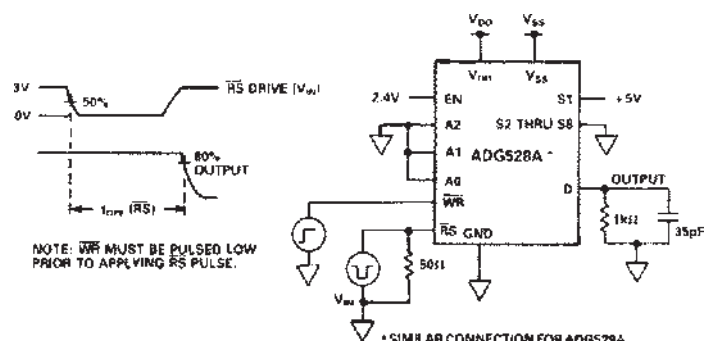
Test Circuit 10. Reset Turn-Off Time, t_{OFF}(RS)
