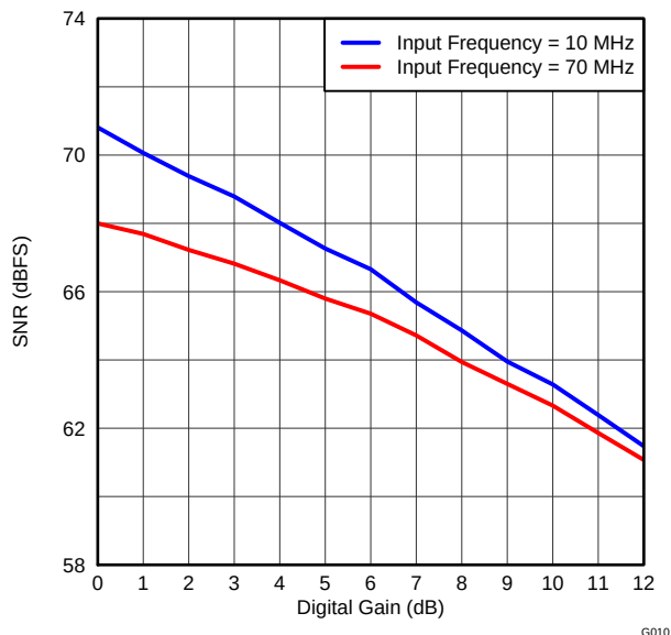
Figure 13. SIGNAL-TO-NOISE RATIO vs DIGITAL GAIN
