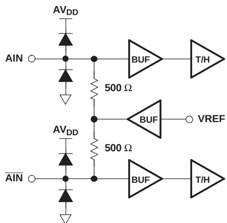
Figure 27. Analog Input
