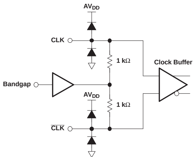
Figure 29. Clock Input
