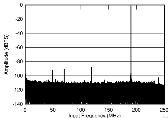
Figure 6-3. FFT for 190-MHz Input Signal
