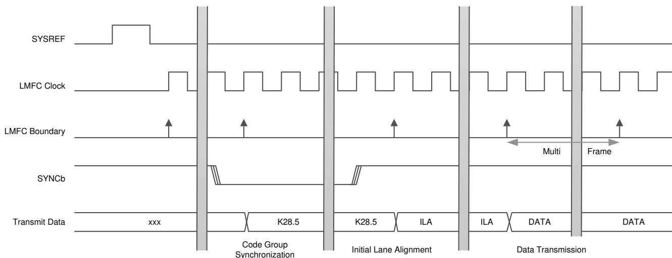
Figure 7-23. ILA Sequence
