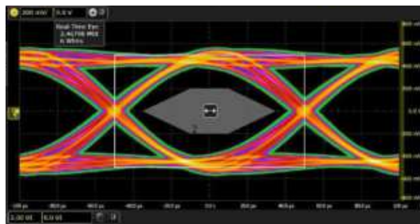
Figure 7-28. Eye at 10-Gbps Bit Rate with Increased Output Swing
