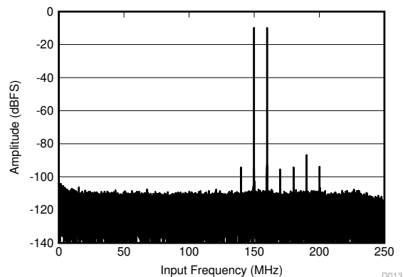
f_{\text{IN1}} = 340\text{ MHz} , f_{\text{IN2}} = 350\text{ MHz} , \text{IMD} = 95.08\text{ dBFS} , each tone at -10\text{ dBFS}
