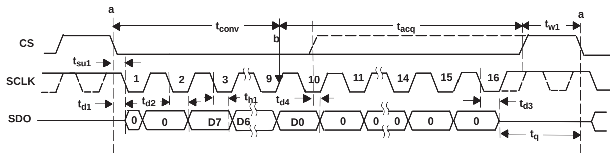
Figure 2. ADS7885 Interface Timing Diagram
