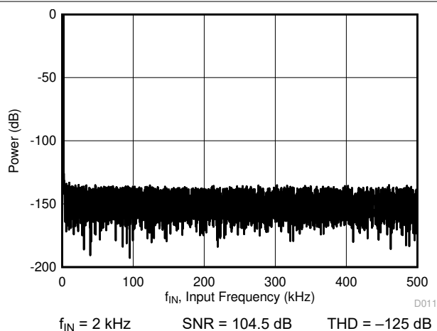
Figure 5-21. Typical FFT - ADS8900B
