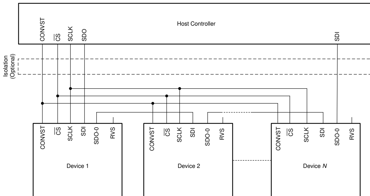
Figure 6-58. Daisy-Chain Connections
