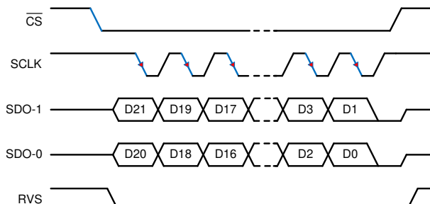
Figure 6-40. SPI-10-D-EDL Protocol
