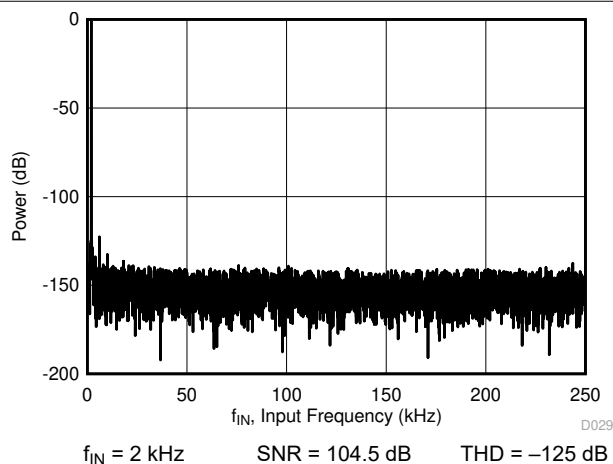
Figure 5-22. Typical FFT - ADS8902B
