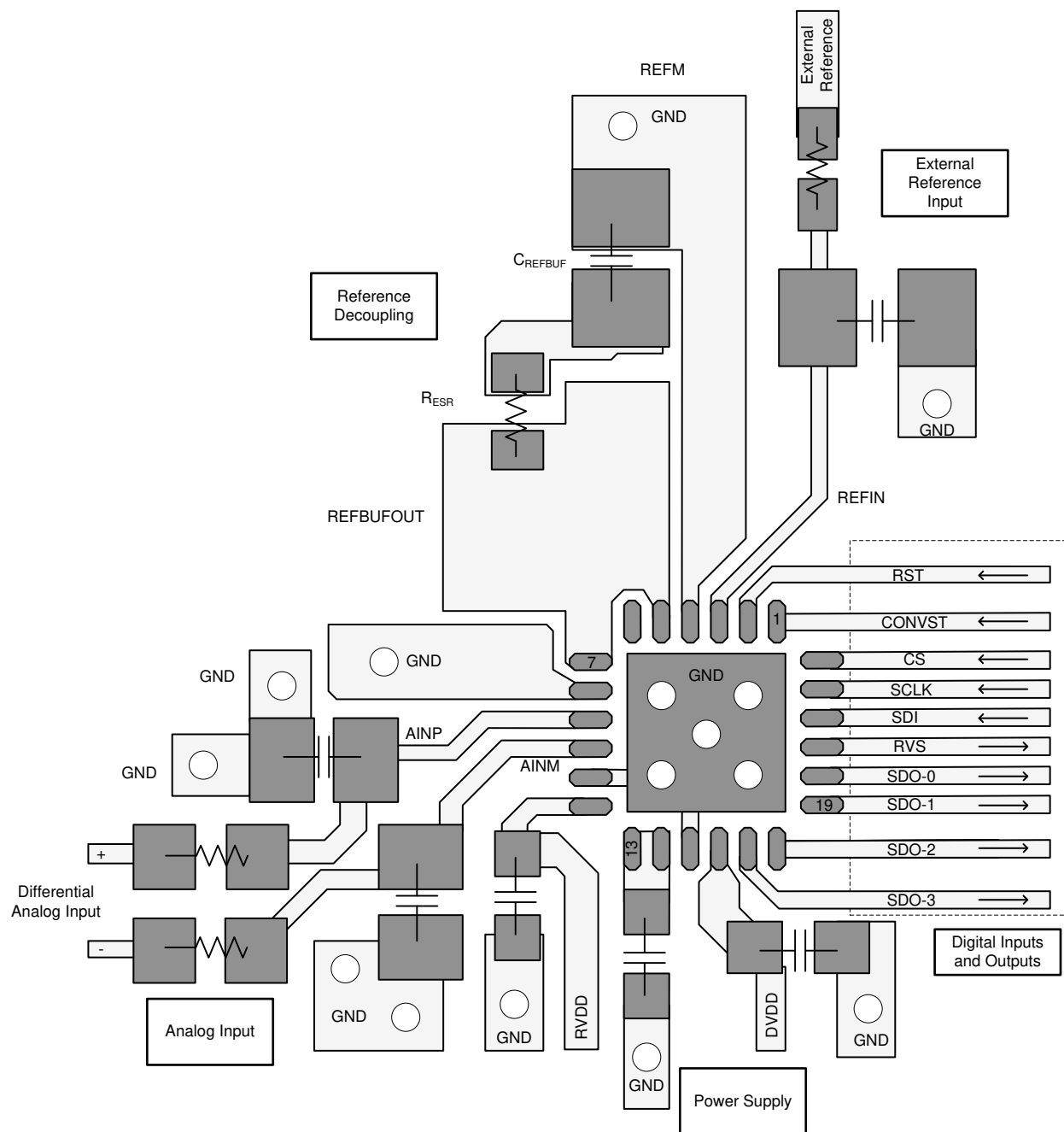
Figure 10-1. Recommended Layout
