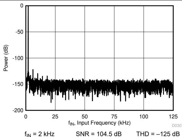
Figure 5-23. Typical FFT - ADS8904B
