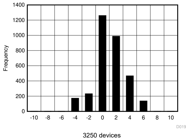
Figure 5-14. Typical Offset Distribution (LSB)
