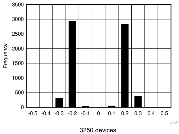
Figure 5-8. Typical DNL Distribution (LSB)
