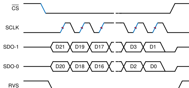
Figure 6-39. SPI-00-D-EDL Protocol
