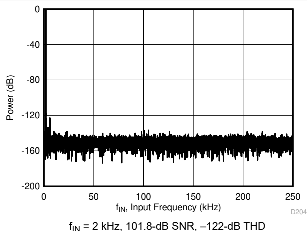
Figure 8-5. Noise-Performance FFT Plot: ADS8902B
