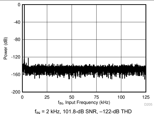
Figure 8-6. Noise-Performance FFT Plot: ADS8904B
