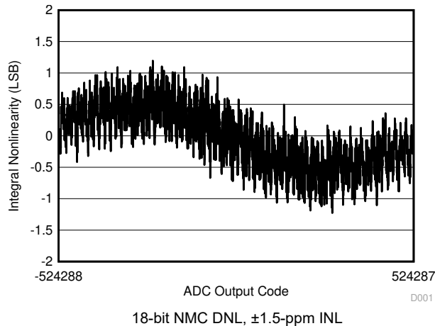
Figure 8-3. Typical Linearity
