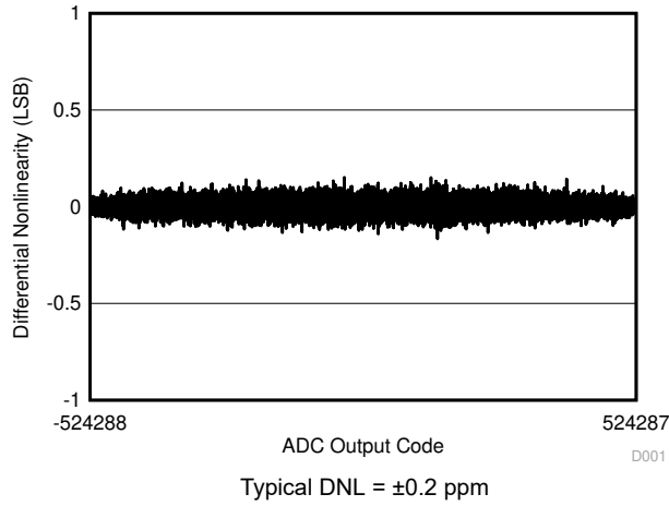
Figure 5-6. Typical DNL
