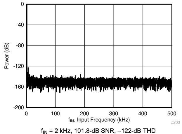
Figure 8-4. Noise-Performance FFT Plot: ADS8900B
