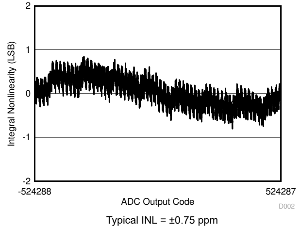
Figure 5-7. Typical INL
