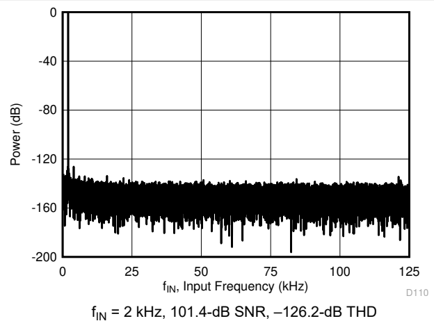
Figure 8-16. Noise-Performance FFT Plot: ADS8904B, Single-Ended Input
