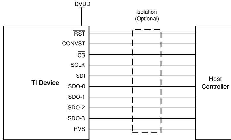
Figure 6-56. MultiSPI Digital Interface, All Pins
