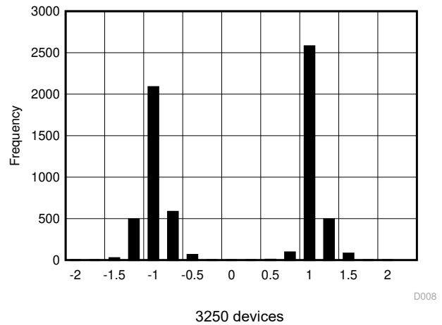
Figure 5-9. Typical INL Distribution (LSB)
