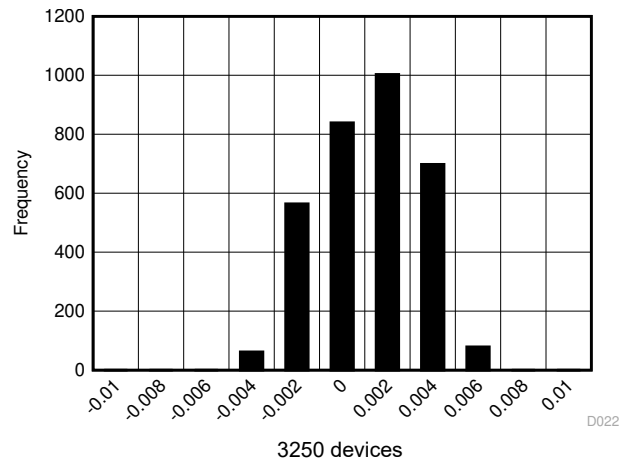
Figure 5-15. Typical Gain Error Distribution (%FS)
