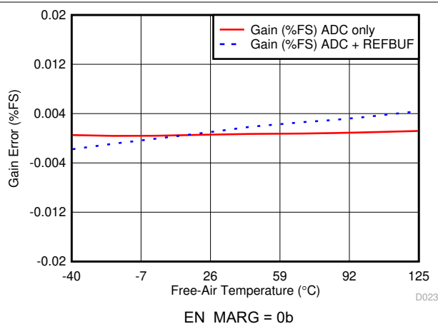
Figure 5-18. Gain Error vs Temperature
