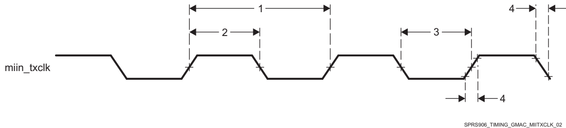
Figure 5-65. Clock Timing (GMAC Transmit) - MII operation
