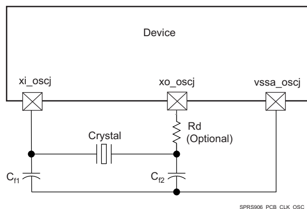
Figure 7-31. Grounding Scheme for High-Frequency Clock
