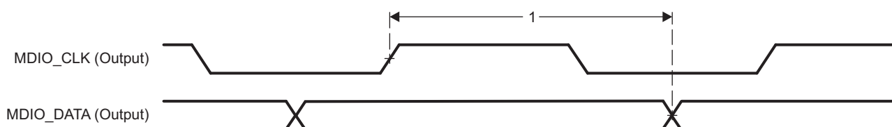
Figure 5-119. PRU-ICSS MDIO_DATA Timing – Output Mode
