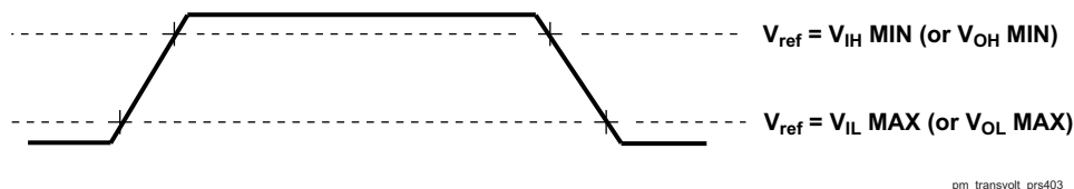
Figure 5-4. Rise and Fall Transition Time Voltage Reference Levels
