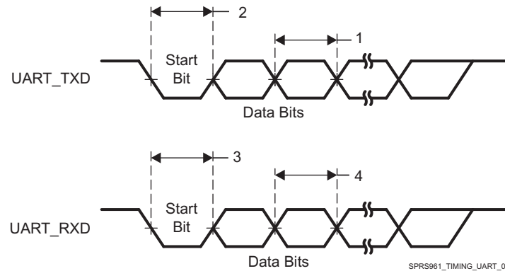
Figure 5-45. UART Timing
