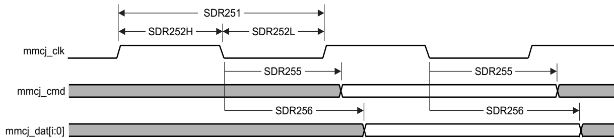
Figure 5-101. MMC/SD/SDIOj in - SDR25 - Transmitter Mode
