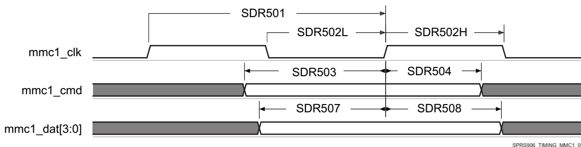
Figure 5-81. MMC/SD/SDIO in - High Speed SDR50 - Receiver Mode
