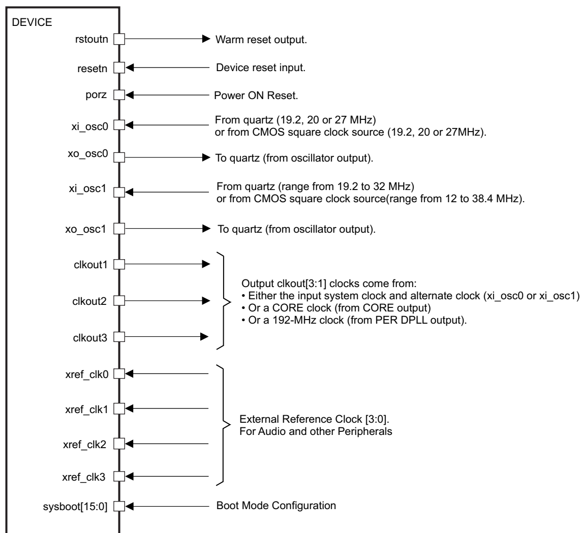
Figure 5-8. Clock Interface
