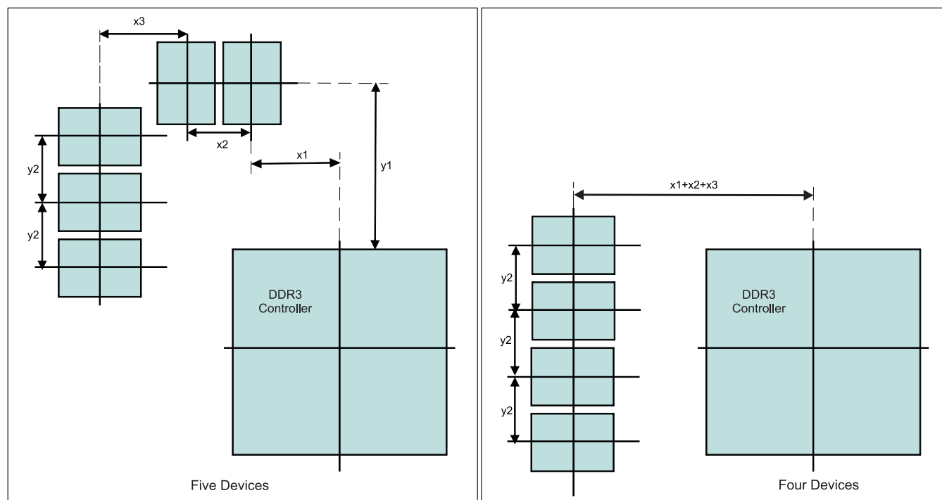
Figure 7-4. Placement Specifications
