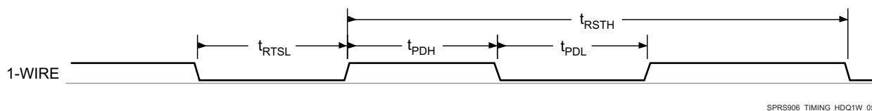
Figure 5-42. 1-Wire—Break (Reset)
