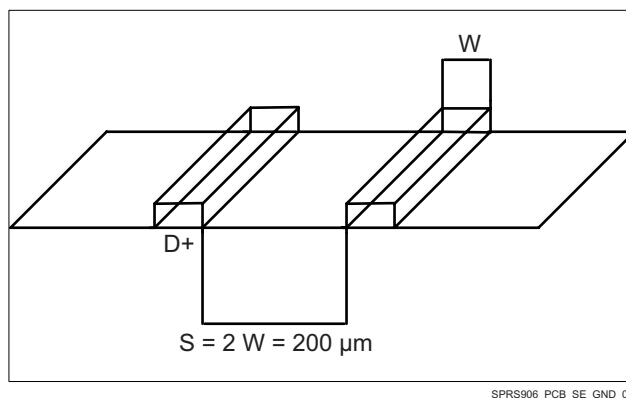
Figure 7-29. Ground Guard Illustration
