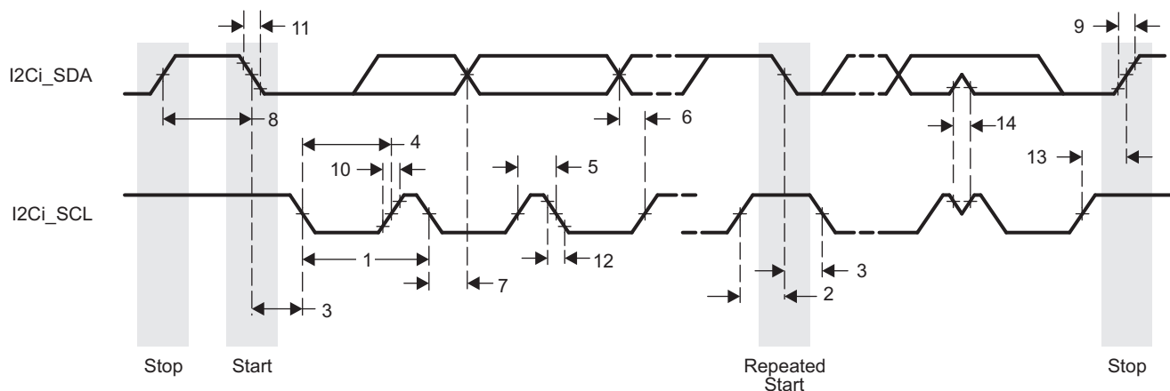
Figure 5-36. I2C Receive Timing
