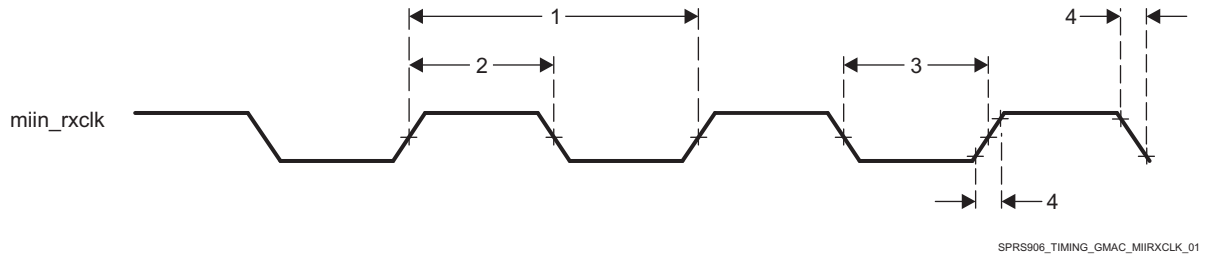
Figure 5-64. Clock Timing (GMAC Receive) - MII operation
