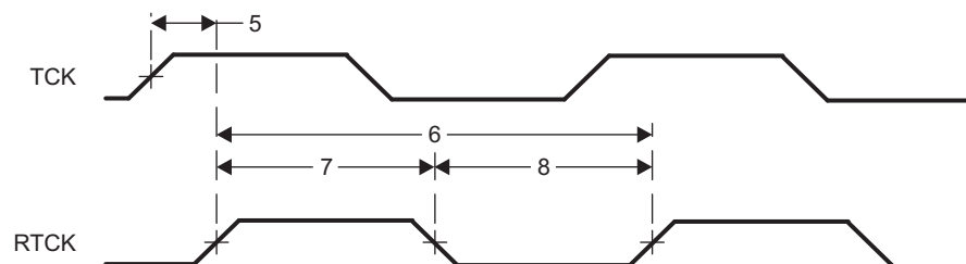
Figure 5-126. JTAG With RTCK Timing
