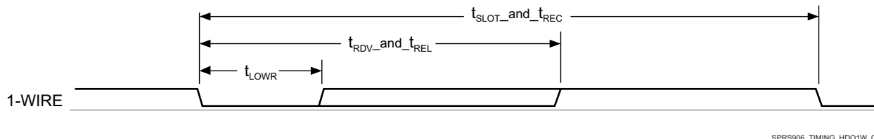
Figure 5-43. 1-Wire—Read Bit (Data)
