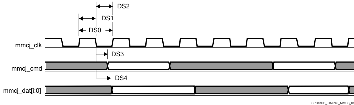
Figure 5-95. MMC/SD/SDIOj in - Default Speed - Transmitter Mode
