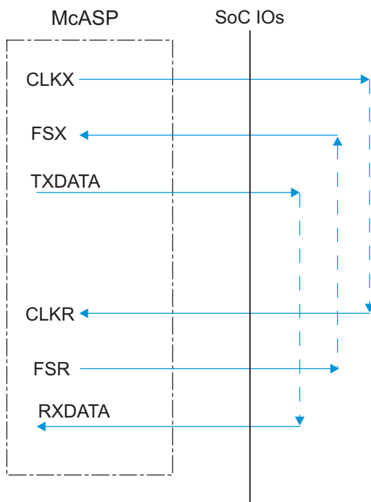
Figure 5-57. McASP1-8 COIFIO – ASYNC Mode
