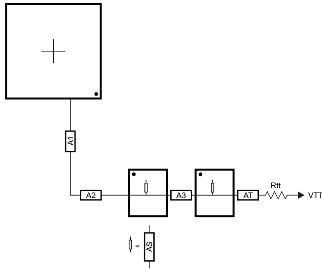
Figure 7-15. ADDR_CTRL Routing for Two Single-Side DDR3 Devices
