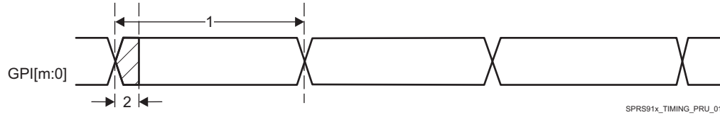
Figure 5-104. PRU-ICSS PRU Direct Input Timing
