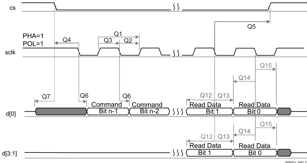
Figure 5-50. QSPI Read (Clock Mode 3)
