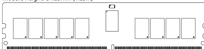
Figure 1: 288-Pin RDIMM (R/C-E1, R/C-E2)
