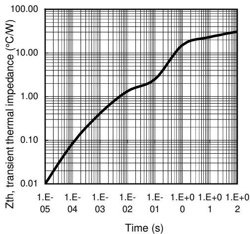
Figure 8 – Transient thermal impedance ( ^{\circ}C/W ) Vs time (s)
