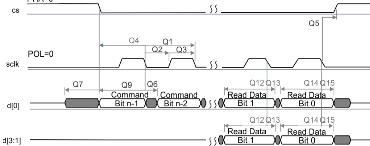
Figure 7-14. QSPI Read (Clock Mode 0)
