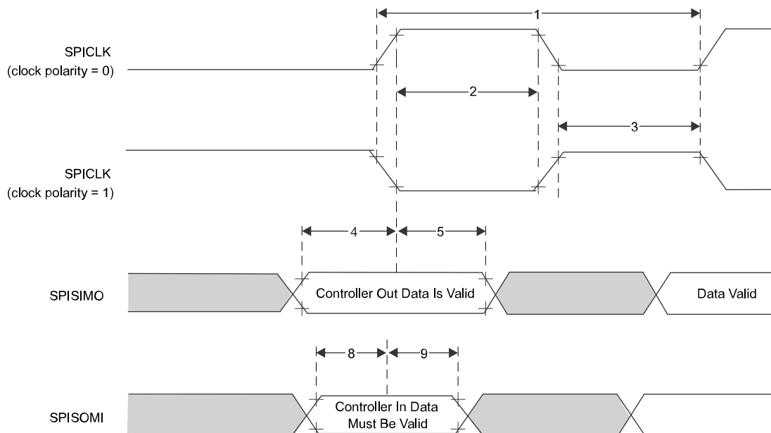
Figure 7-6. SPI Controller Mode External Timing (CLOCK PHASE = 1)
