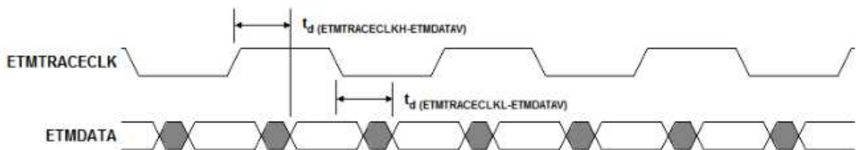
Figure 7-20. ETMDATA Timing
