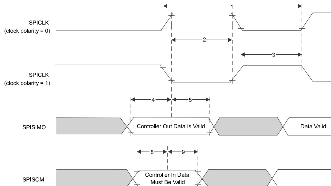
Figure 7-9. SPI Controller Mode External Timing (CLOCK PHASE = 1)
