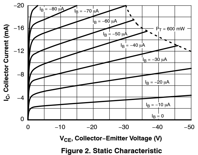
Figure 2. Static Characteristic
