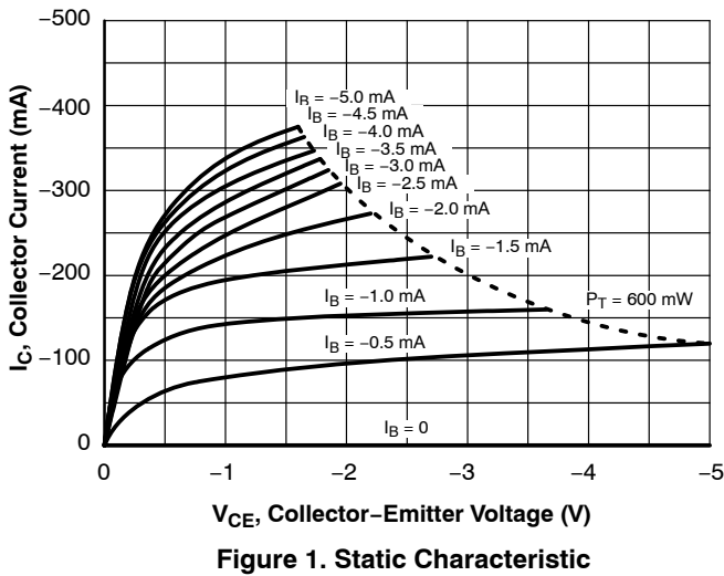
Figure 1. Static Characteristic
