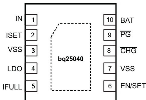
10-Pin 2mm × 3mm DFN (TOP VIEW)
