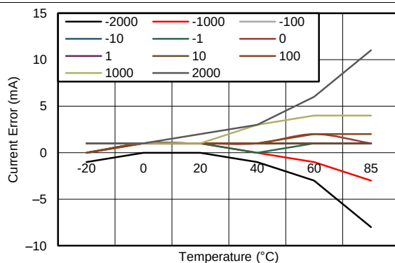
Figure 24. Current Error vs. Temperature
