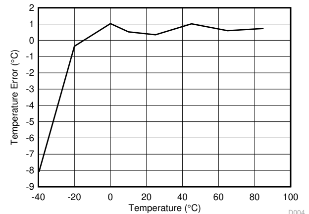
Figure 8-8. T_{Err}
