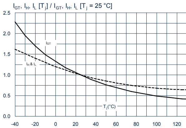
Figure 7. Relative variation of gate trigger current, holding and latching current versus junction temperature (typical values)
