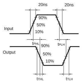
Fig.2 Switching characteristics
