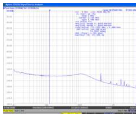
Reference: Crystal Closed-Loop Phase 24.576-MHz Input 25 MHz Noise from 2.4576- GHz VCO LVCMOS
