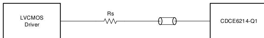
Figure 6-9. Single-Ended LVC MOS to Reference
