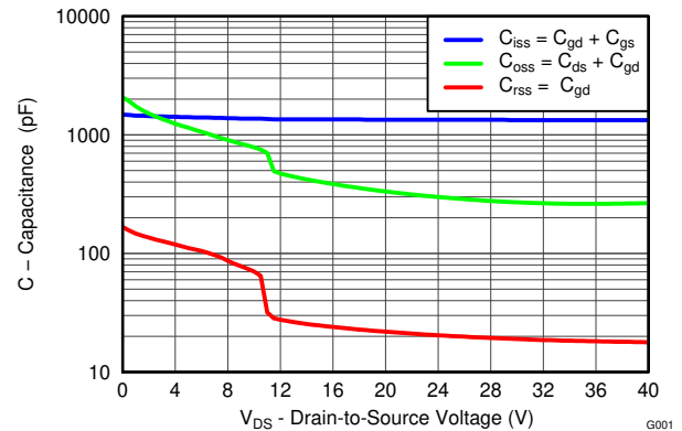
Figure 4-5. Capacitance
