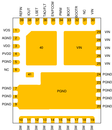
Pin Functions
