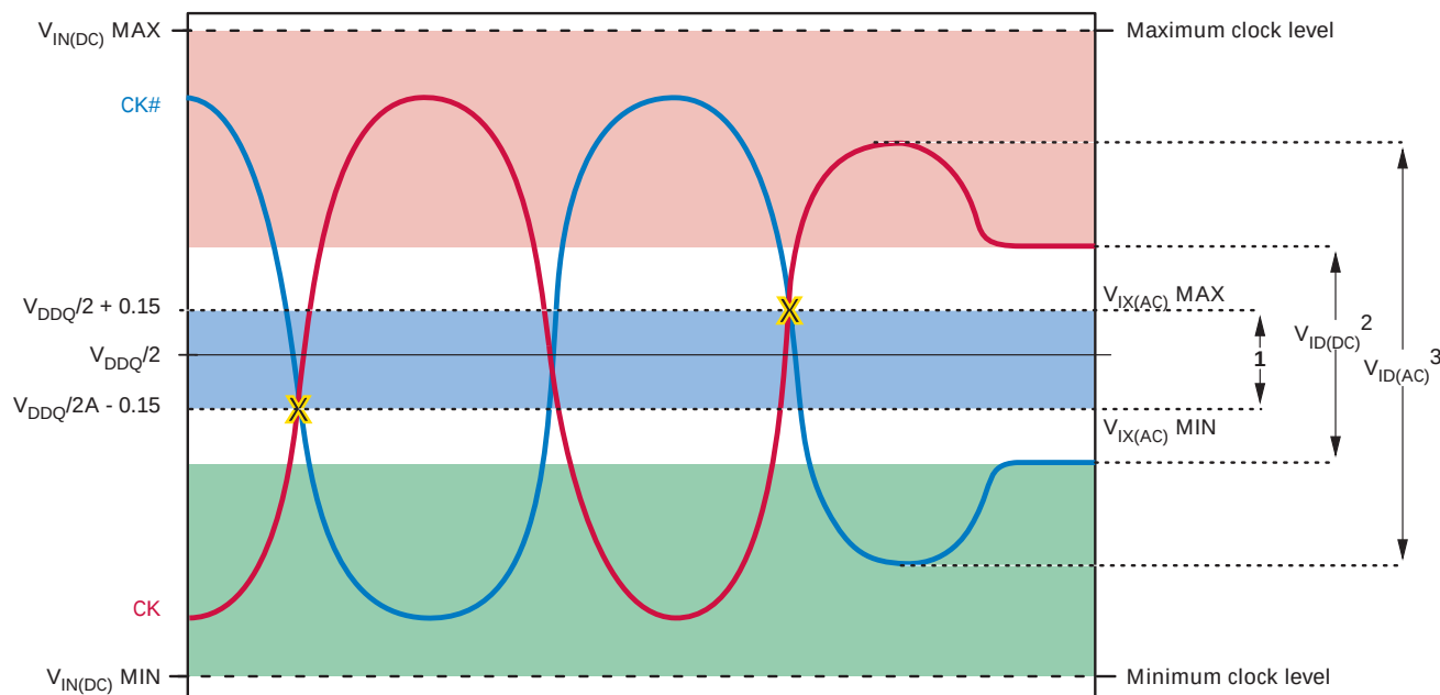
Figure 7: Clock Input
