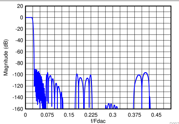
Figure 7-20. Composite Magnitude Response for 20x Interpolation
