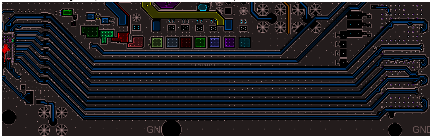
Figure 8-10. Layout Example of High Speed SerDes Traces
