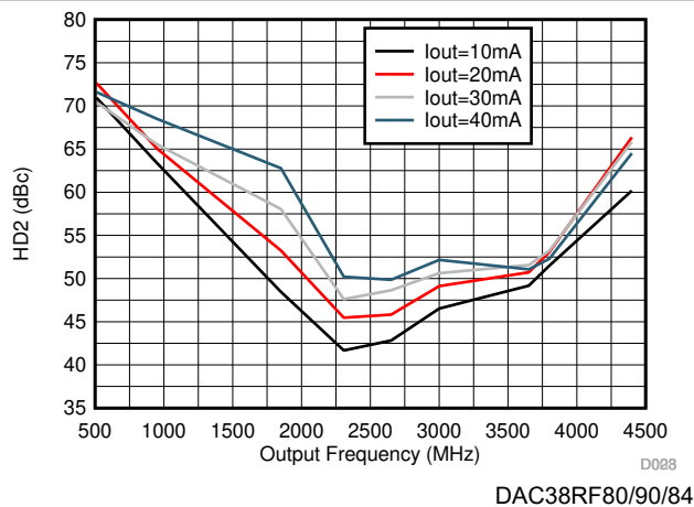
Figure 6-10. HD2 vs Output Frequency Over Output Current I_{\text{outFS}}
