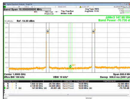
2x20-MHz LTE at 1.84 GHz and 2.14 GHz, 800 MHz Span
