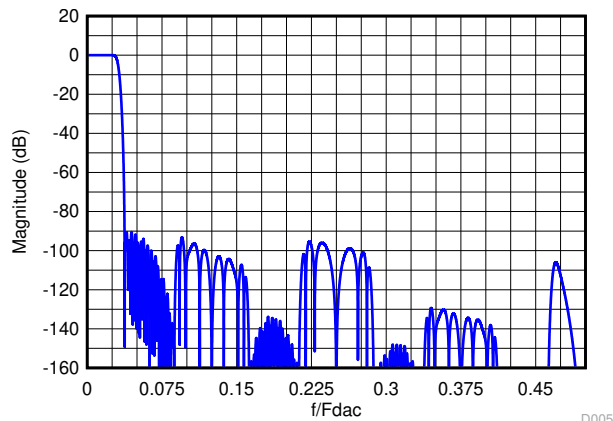
Figure 7-18. Composite Magnitude Response for 16x Interpolation
