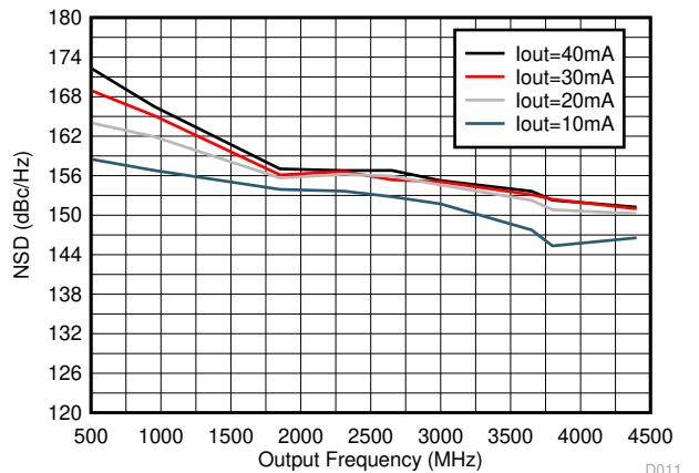
Figure 6-3. NSD vs Output Frequency Over Output Current I_{\text{outFS}}
