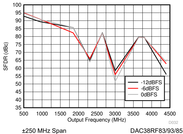
Figure 6-25. SFDR vs Output Frequency Over Input Scale
