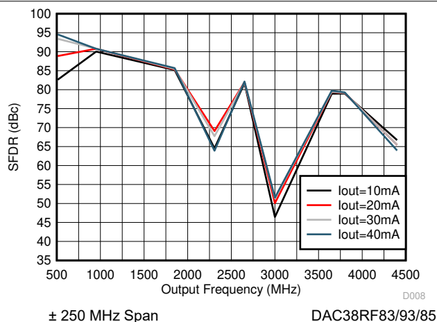
Figure 6-27. SFDR vs Output Frequency Over Output Current I_{\text{outFS}}
