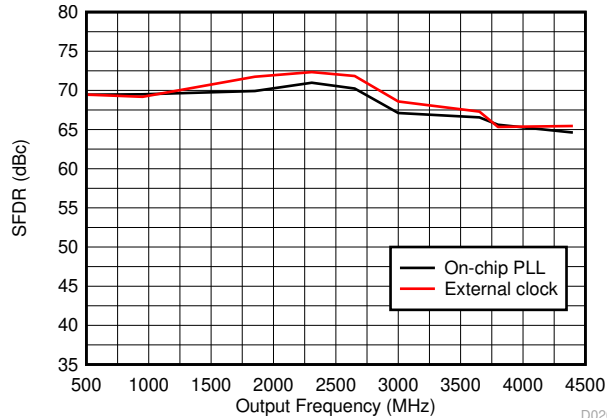
Figure 6-23. SFDR vs Output Frequency Over Clocking Option
