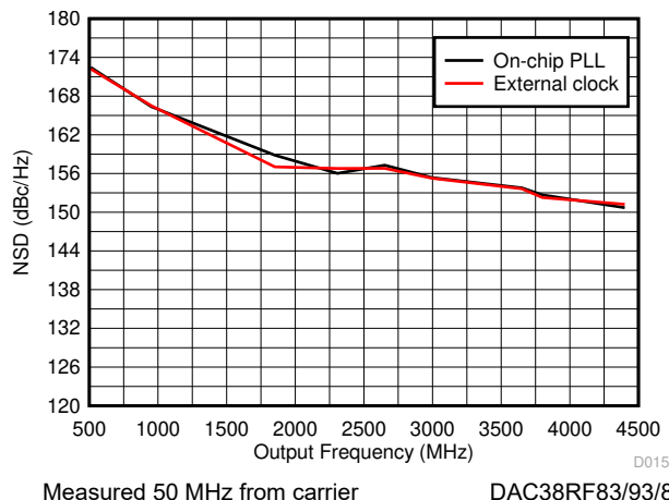
Figure 6-5. NSD vs Output Frequency Over Clocking Option
