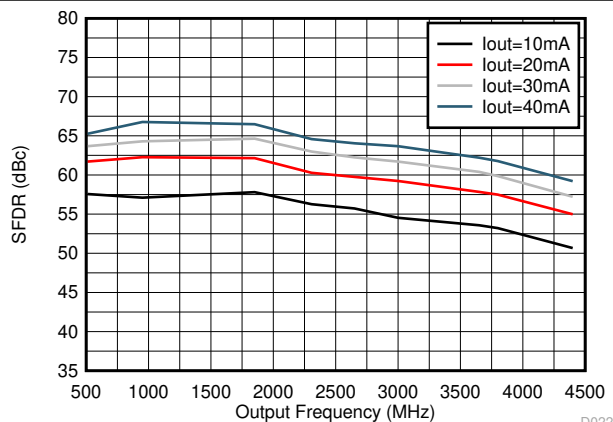
D022 Excludes HD2, HD3 and CMP2 DAC38RF80/90/84
