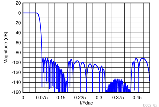
Figure 7-15. Composite Magnitude Response for 8x Interpolation
