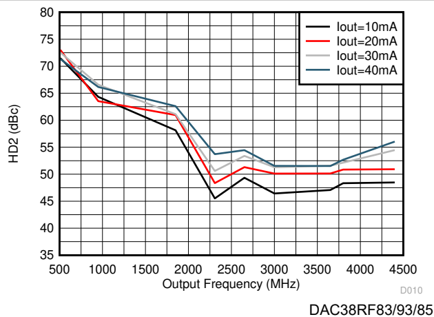
Figure 6-9. HD2 vs Output Frequency Over Output Current I_{\text{outFS}}
