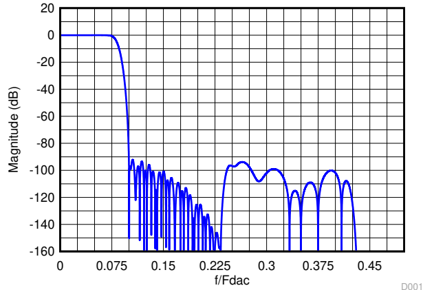
Figure 7-14. Composite Magnitude Response for 6x Interpolation
