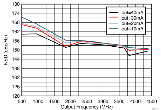
Figure 6-4. NSD vs Output Frequency Over Output Current I_{\text{outFS}}
