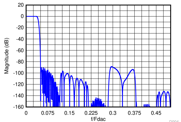
Figure 7-17. Composite Magnitude Response for 12x Interpolation
