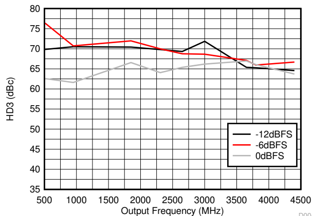
D004 DAC38RF83/93/85
