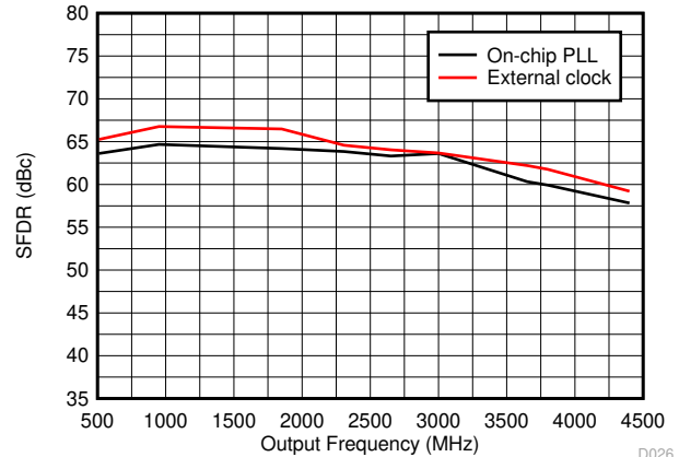
Figure 6-24. SFDR vs Output Frequency Over Clocking Option
