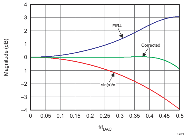
Figure 7-23. Composite Magnitude Spectrum for INVSINC
