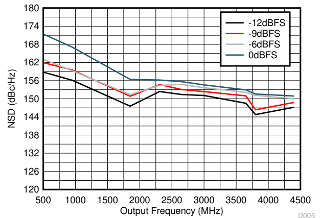
Figure 6-2. NSD vs Output Frequency Over Input Scale
