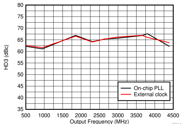
D014 DAC38RF83/93/85
