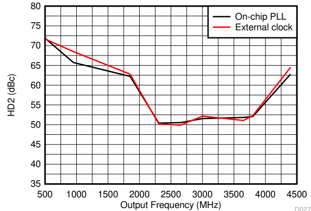
D027 DAC38RF80/90/84
