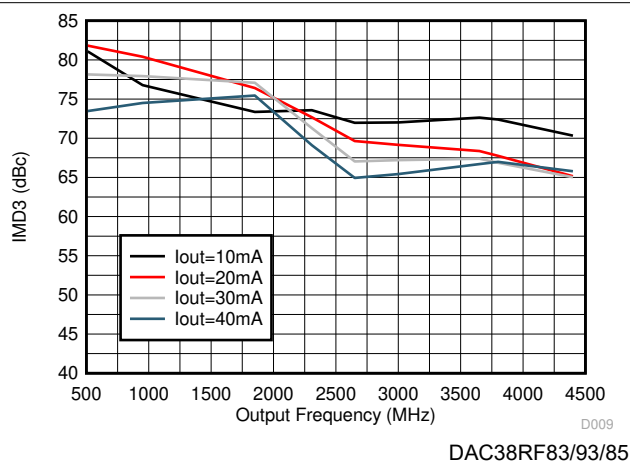
Figure 6-33. IMD3 vs Output Frequency Over Output Current I_{\text{outFS}}
