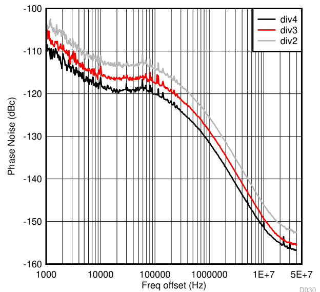
Figure 6-42. VCO1 Output Clock Phase Noise vs Offset frequency Over Divider Ratio
