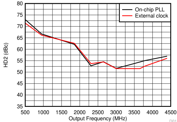
D013 DAC38RF83/93/85
