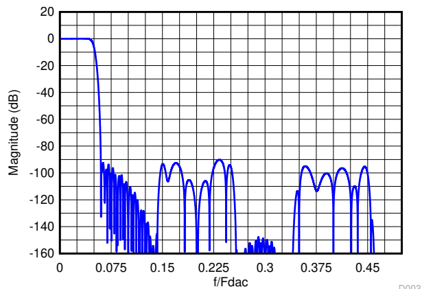
Figure 7-16. Composite Magnitude Response for 10x Interpolation
