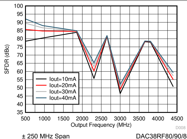
Figure 6-28. SFDR vs Output Frequency Over Output Current I_{\text{outFS}}
