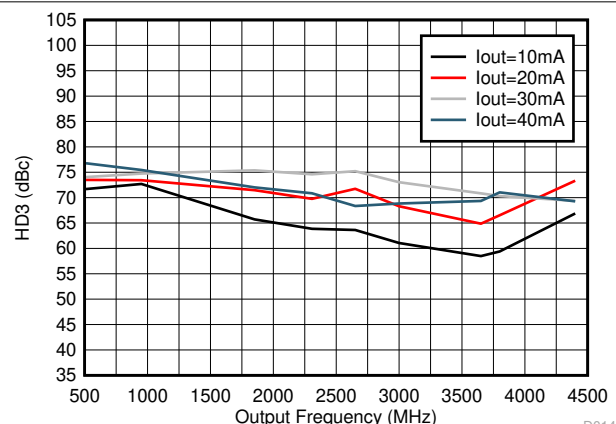
D014 DAC38RF80/90/84
