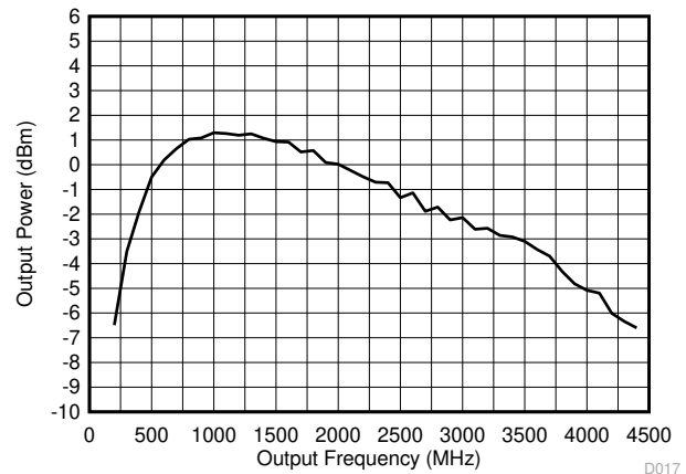
D017 DAC38RF80/90/84
