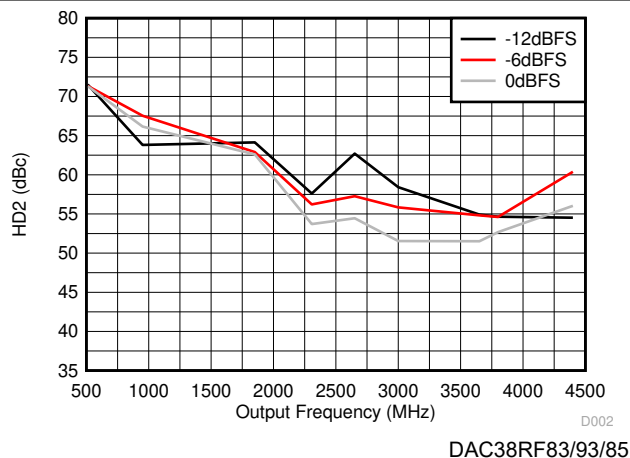
Figure 6-7. HD2 vs Output Frequency Over Input Scale
