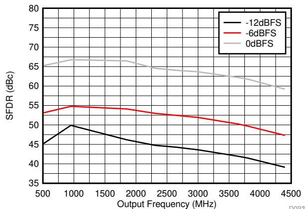
D082 Excludes HD2, HD3 and CMP2 DAC38RF80/90/84
