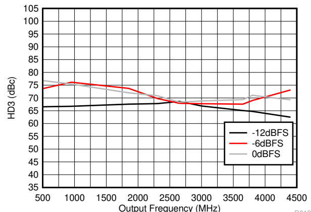
D013 DAC38RF80/90/84
