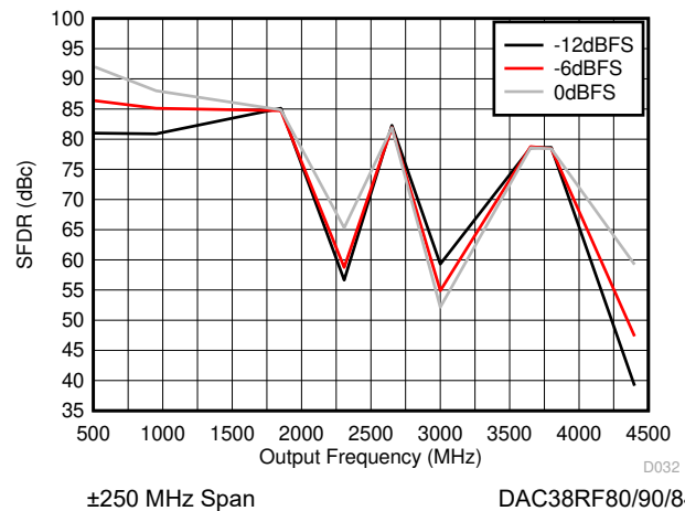
Figure 6-26. SFDR vs Output Frequency Over Input Scale
