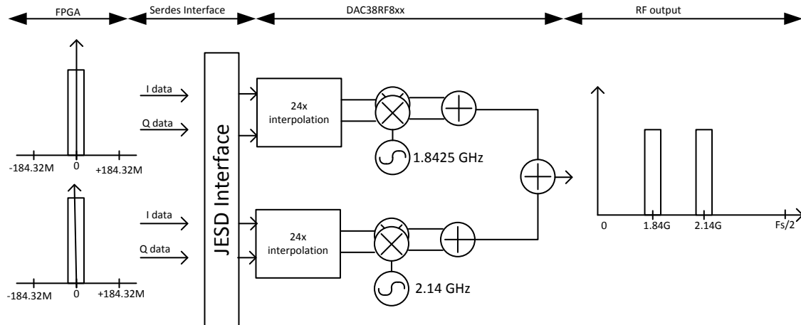
Figure 8-3. Dual Band LTE Downlink Transmitter Block Diagram
