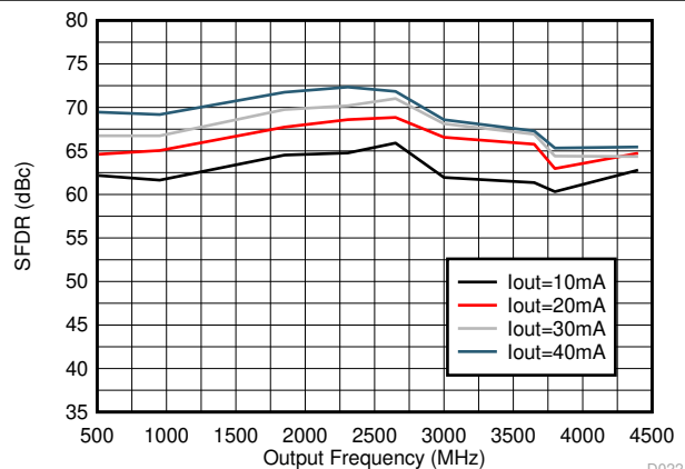
D022 Excludes HD2, HD3 and CMP2 DAC38RF83/93/85
