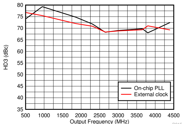
D015 DAC38RF80/90/84
