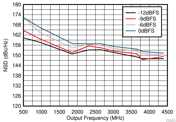
Figure 6-1. NSD vs Output Frequency Over Input Scale
