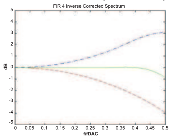
Figure 24. Magnitude Spectrum for FIR4
