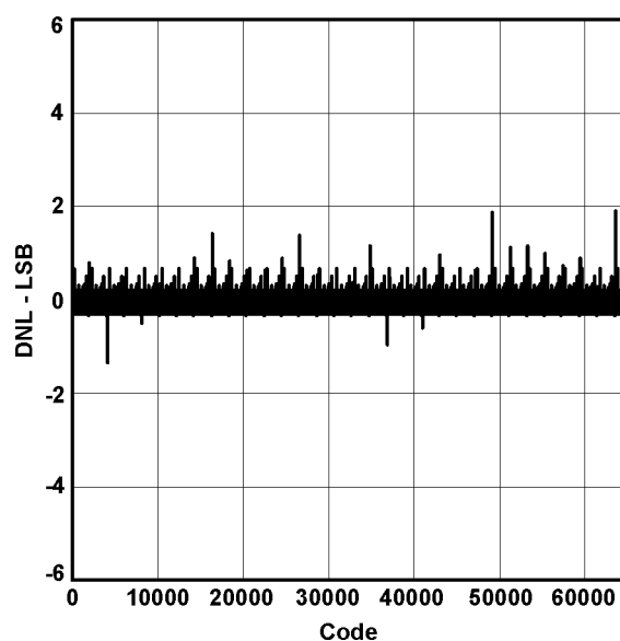
Figure 2. Differential Nonlinearity
