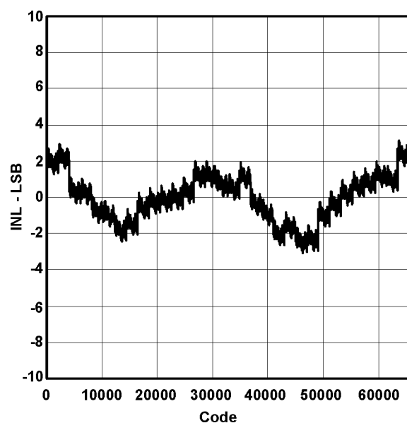
Figure 1. Integral Nonlinearity
