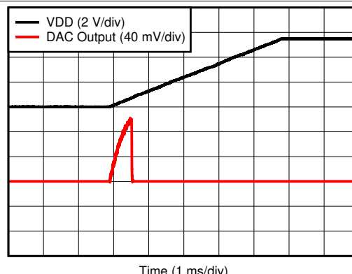
Figure 40. Power-On Glitch
