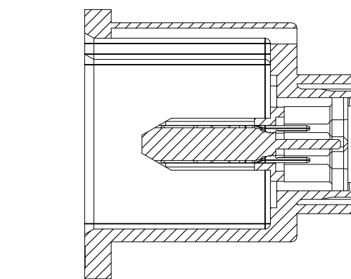
SECT B-B
