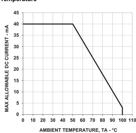
Figure 8: Maximum Forward Current vs. Ambient Temperature
