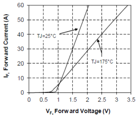
Figure 18 • Forward Characteristics
