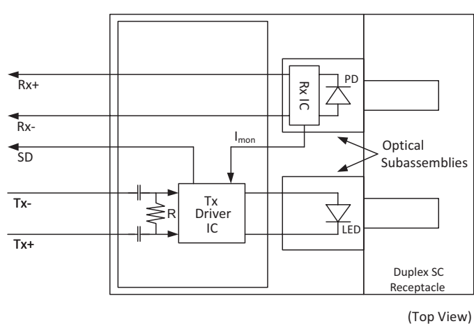
Figure 2: Block Diagram 1 × 9 SC Transceiver
