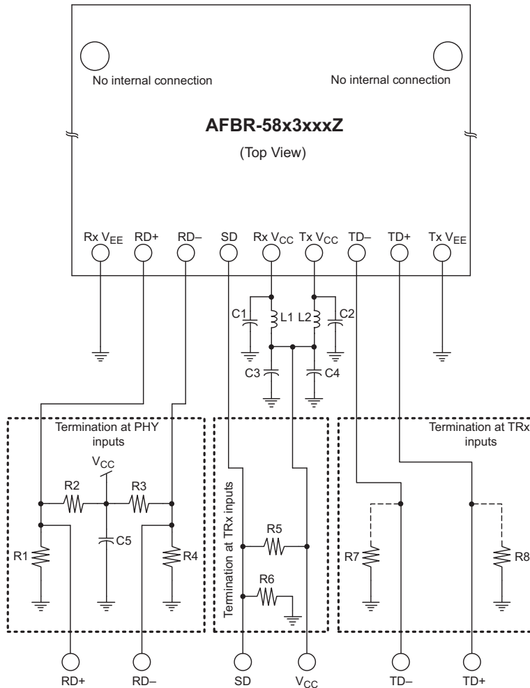
Figure 10: Recommended Decoupling and Termination Circuits
