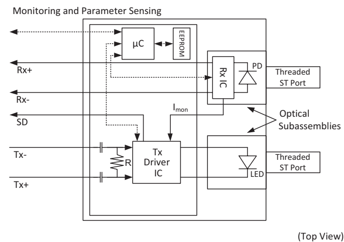
Figure 3: Block Diagram 2 × 9 ST Transceiver
