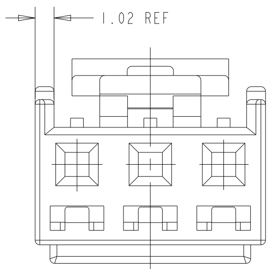
FRONT VIEW (3 POSITION SHOWN)
