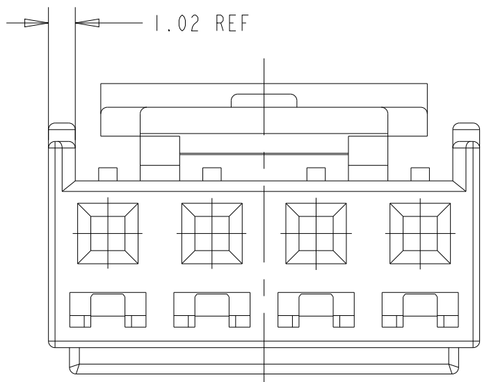
FRONT VIEW (4 POSITION SHOWN)
