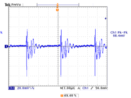
High Line, Full Load Ripple noise=98.4mV
