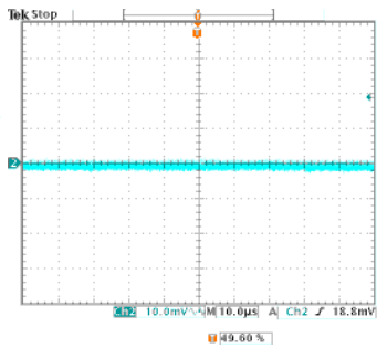
Normal Line, Full Load Ripple current= (3.2/10) \times 10=3.2\text{mA}
