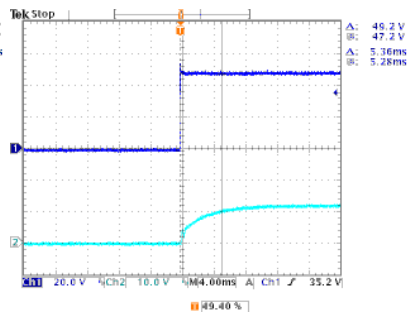
Normal Line, Full Load Delay Time=5.36mS
