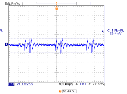
High Line, Full Load Ripple noise=30.4mV
