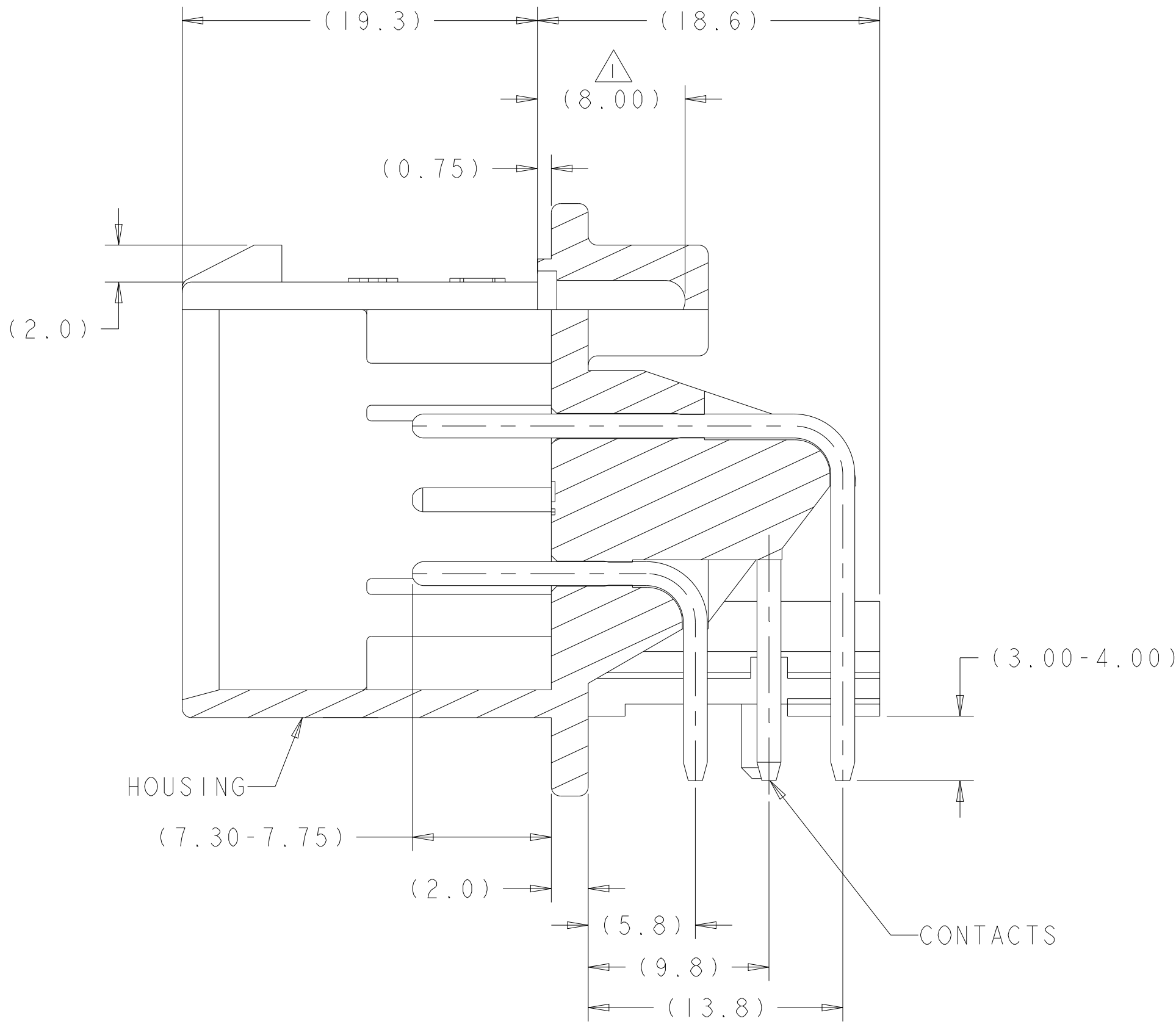
SECTION B-B
