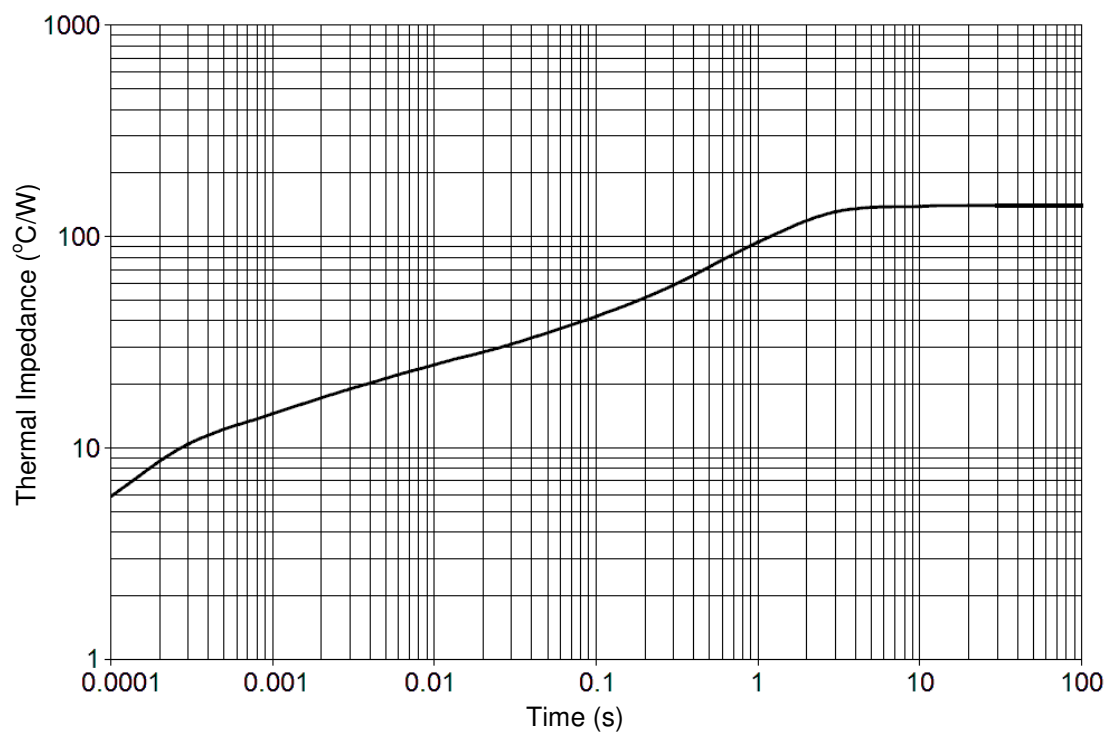
FIGURE 3 Maximum Thermal Impedance at T_L = 25\text{ °C}
