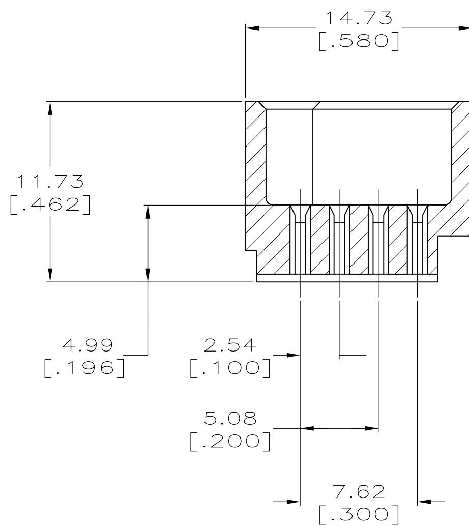
SECTION T-T
