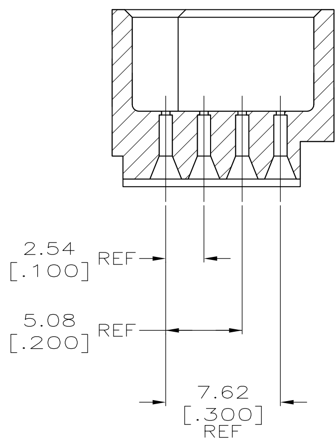
SECTION S-S
