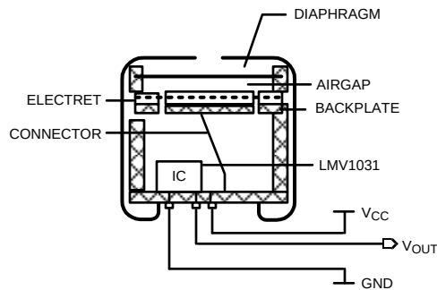
Figure 10. Built-in Gain
