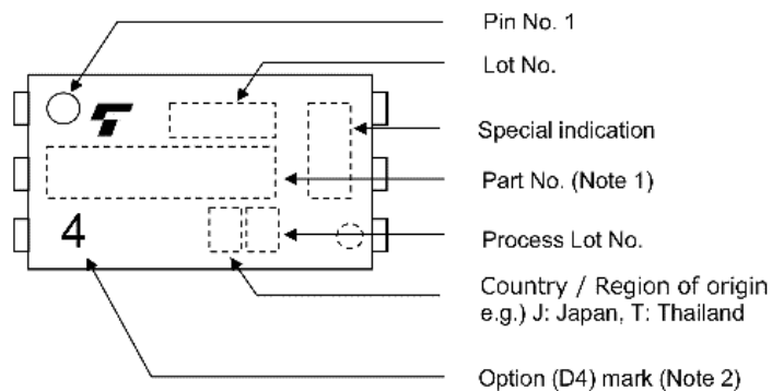
Fig. 17.4 Marking Example
