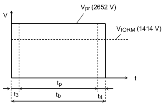
Figure 2 Partial discharge measurement procedure according to EN IEC 60747 Non-destructive test for 100 % inspection.
