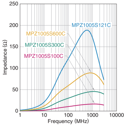
MPZ1005S series
