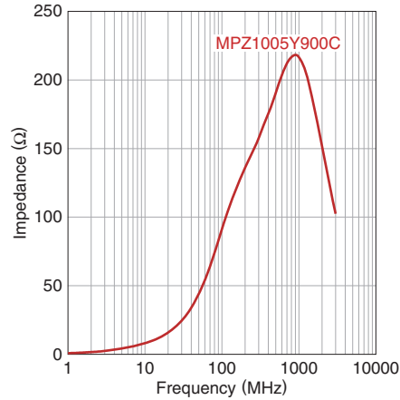
MPZ1005Y series
