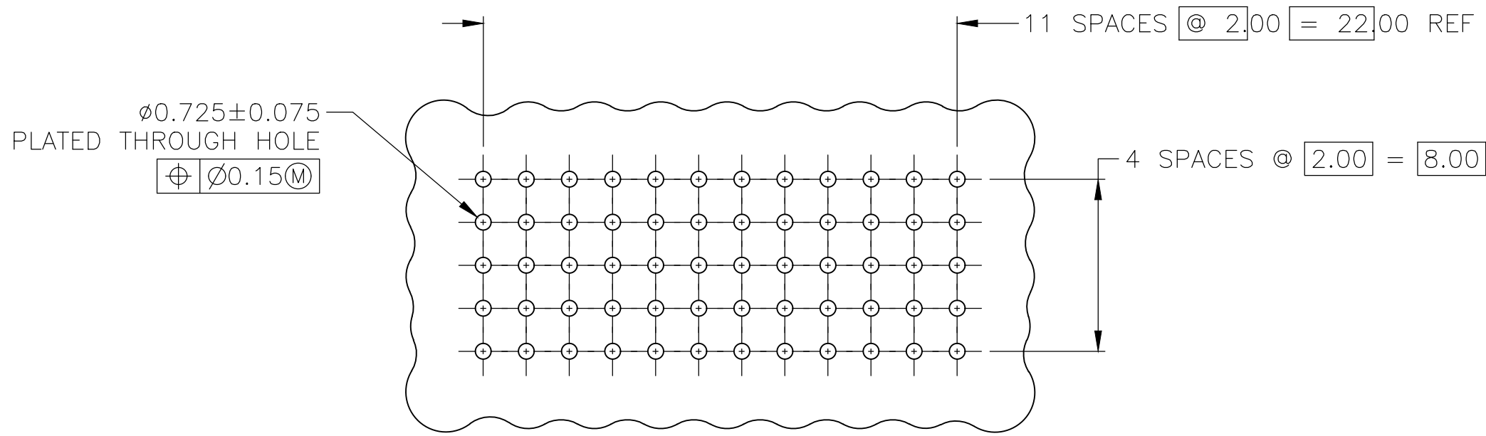
RECOMMENDED CIRCUIT PATTERN (COMPONENT SIDE)
